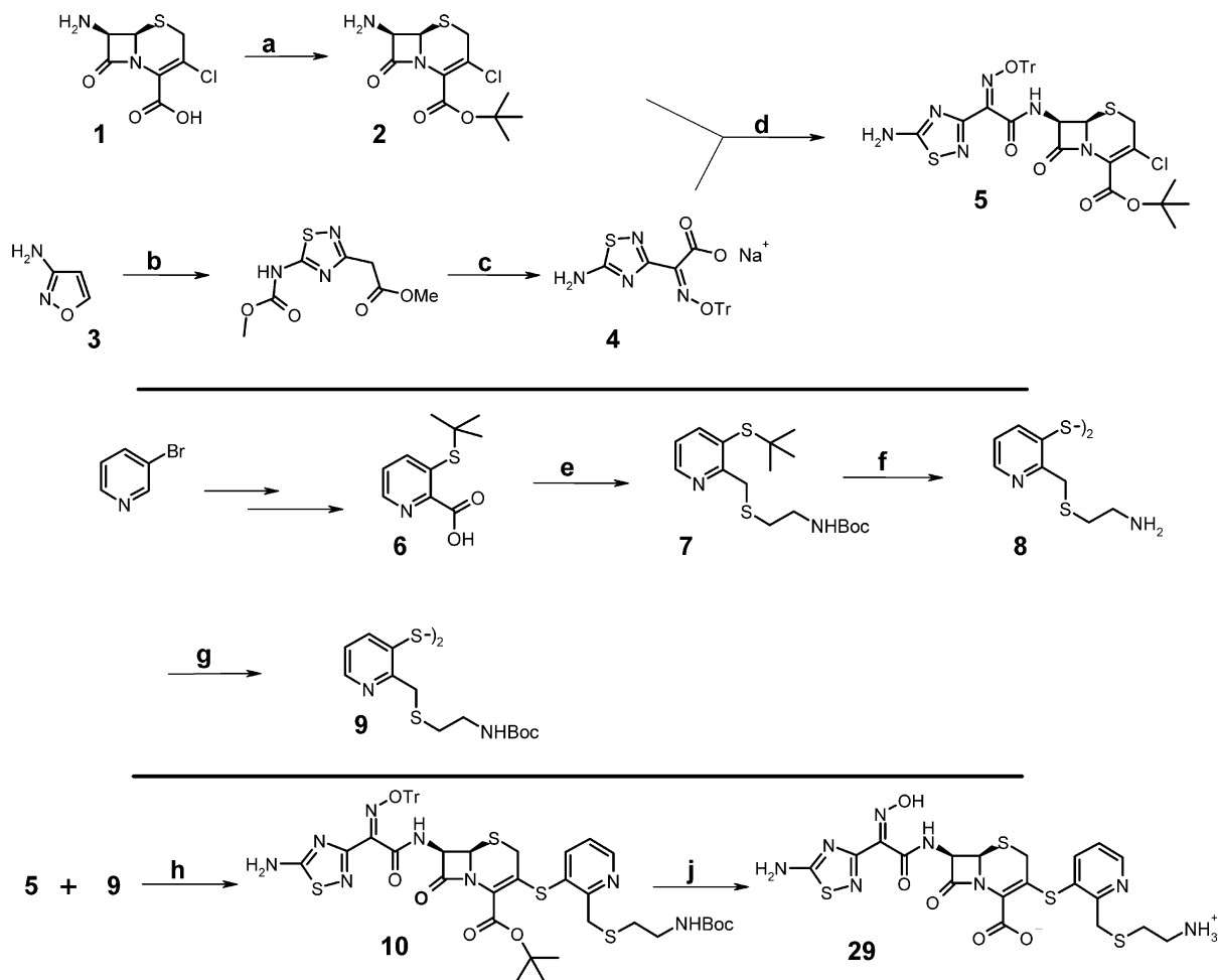
Scheme 1. (a) t -BuOAc, \text{BF}_3 \cdot \text{Et}_2\text{O} ; (b) (i) KSCN, \text{MeOC(O)Cl} ; (ii) MeOH, 60°; (iii) peracetic acid; (iv) MeOH, \text{SOCl}_2 ; (c) (i) \text{Br}_2 , MeOH; (ii) pyridine N -oxide, acetonitrile; (iii) \text{NH}_2\text{OH} , EtOH; (iv) trityl chloride, \text{Et}_3\text{N} , DMF; (v) NaOH, EtOH, water; (d) (\text{PhO})_2\text{P(O)Cl} , 2,6-lutidine, THF; (e) (i) \text{ClC(O)OEt} , \text{Et}_3\text{N} ; (ii) \text{NaBH}_4 , THF; (iii) \text{SOCl}_2 , DMF; (iv) N -Boc-cysteamine; (f) (i) 6M HCl; reflux; (ii) air, water; (g) Boc-anhydride, \text{Et}_3\text{N} , ethyl acetate, MeOH; (h) \text{Ph}_3\text{P} , \text{NaHCO}_3 , DMF, water; (j) (i) trifluoroacetic acid, triethylsilane, \text{CH}_2\text{Cl}_2 ; (ii) HP20 resin, acetonitrile/water.
