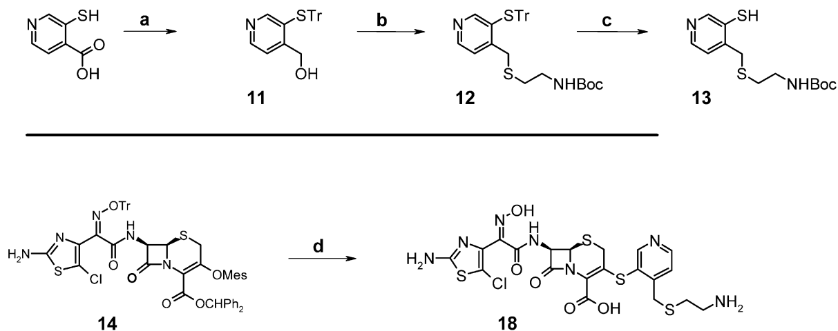
Scheme 2. (a) (i) B 2 H 6 , THF; (ii) TrCl, Et 3 N, DMF; (b) (i) SOCl 2 , DMF; (ii) HSCH 2 CH 2 NHC(O)O- t -Bu, DMF, K 2 CO 3 ; (c) (i) trifluoroacetic acid, triethylsilane, CH 2 Cl 2 ; (ii) di- t -butyldicarbonate, (iPr) 2 NEt; (iii) sodium methoxide, MeOH; (d) (i) 13 , ethyl acetate; (ii) trifluoroacetic acid, triethylsilane, CH 2 Cl 2 .
